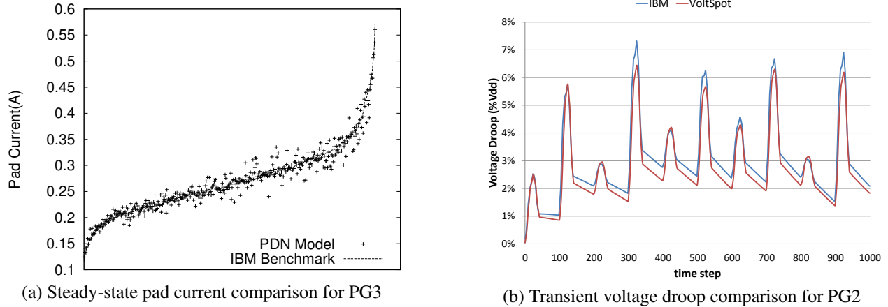
Figure 4: Current/Voltage comparison between IBM data and VoltSpot results.
